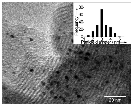
Figure 1. TEM image of 5% Pt/MCM-41. Inset: Particle size distribution.
